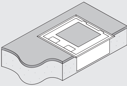
FFOB-188 Stainless Steel lid with 14mm Rebate
